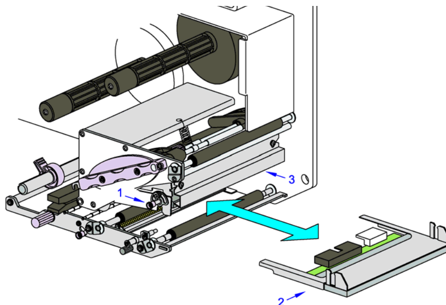
Figure 6-2, Print Head Replacement
